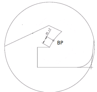
Figure 2 - The Gabarit has a marked BP-point (buckle point left & right) as specified in UN Regulation No. 16 (Annex 17 - Appendix 1)
