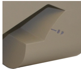
Figure 2 - The Gabarit has a marked BP-point (buckle point left & right) as specified in UN Regulation No. 16 (Annex 17 - Appendix 1)
